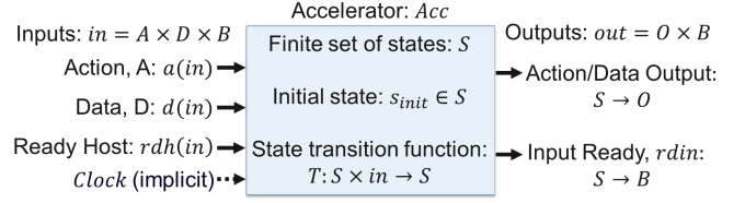
Fig. 3. Accelerator transition system model (Def. 1).
