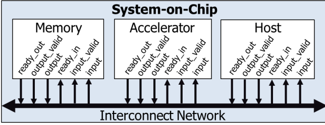
Fig. 1. Accelerator model in this paper.
