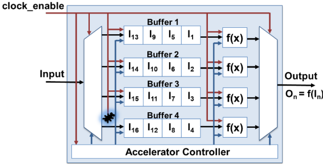
Fig. 2. Bug example: clock\_enable disconnected from Buffer 4.
